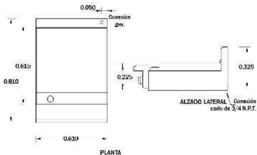
Modelo: FR-P24C
