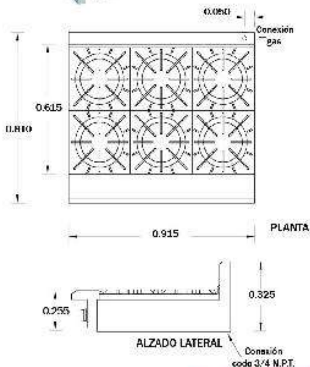
Modelo: FR-6C
