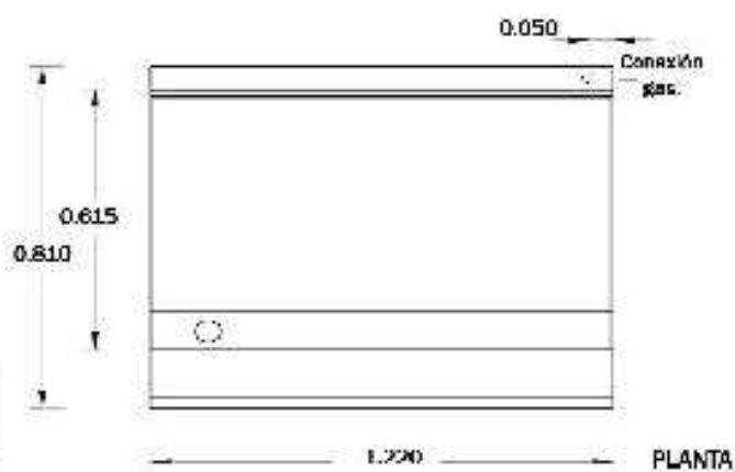
Modelo: FR-P48C
